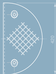
Plan Elevation (Shoulder Ramp)
